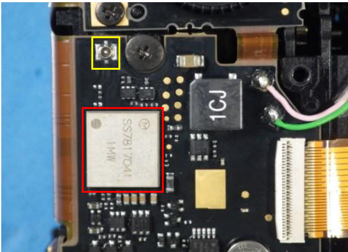
4 Main Board Circuit with Battery Case Block (Magnified)
