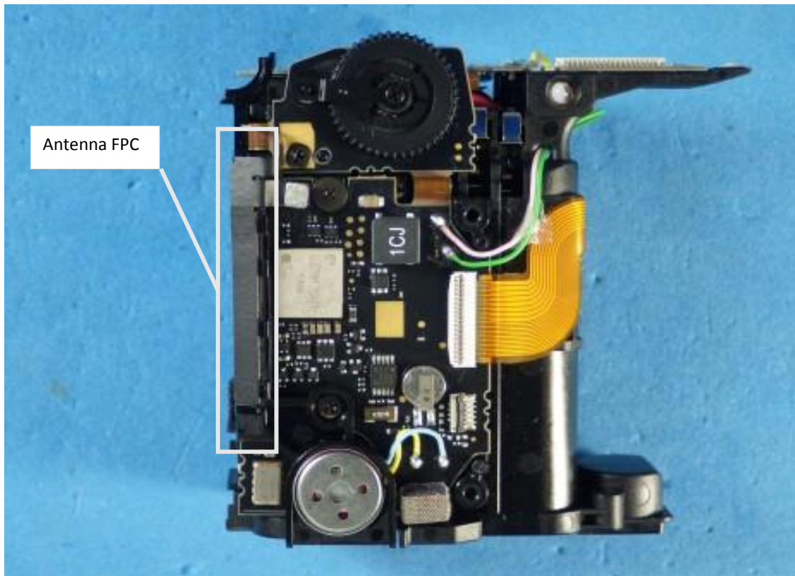
7 Antenna FPC with Main Board Circuit
