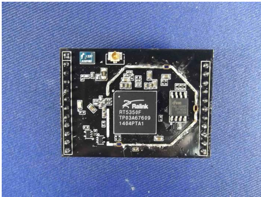
The EUT-Front View (Without Shielding)
