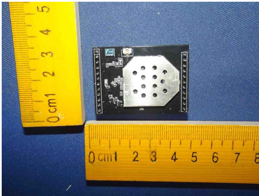
The EUT-Front View (With Shielding)
