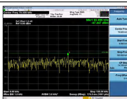
Band66-15MHz-16QAM-132047-75RB#0-0.009~ 0.15-PASS
