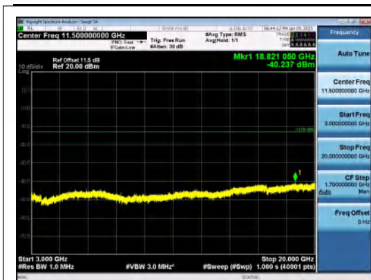
Band66-15MHz-16QAM-132047-1RB#74-3000~ 20000-PASS
