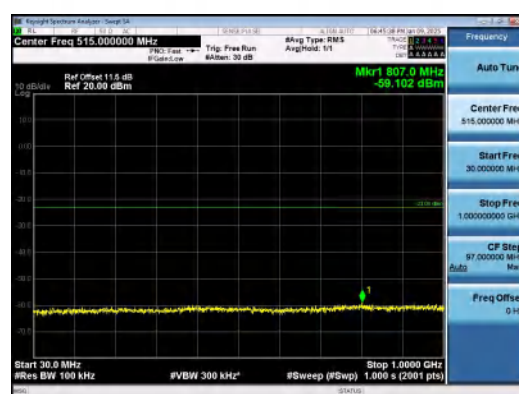
Band66-15MHz-16QAM-132047-75RB#0-30~10 00-PASS
