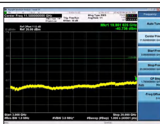
Band66-20MHz-16QAM-132072-1RB#0-3000~20000-PASS
