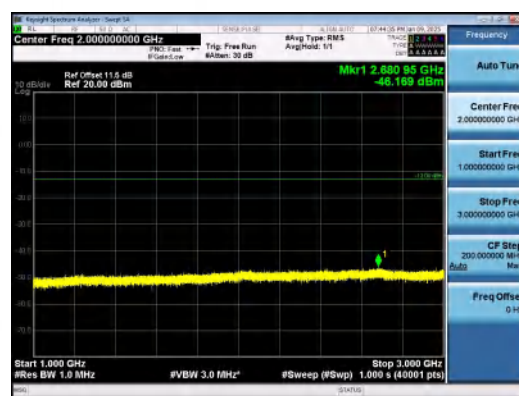
Band66-20MHz-16QAM-132072-1RB#99-1000~3000-PASS
