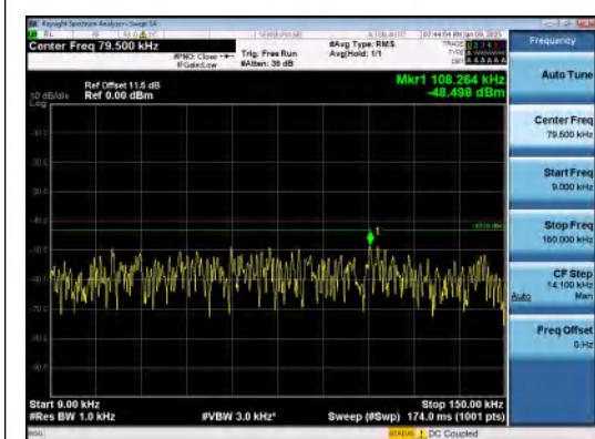
Band66-20MHz-16QAM-132072-1RB#99-0.009~0.15-PASS
