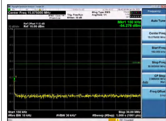
Band66-15MHz-16QAM-132047-75RB#0-0.15~3 0-PASS
