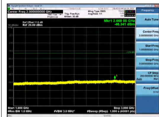
Band66-15MHz-16QAM-132047-75RB#0-1000~ 3000-PASS
