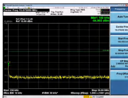
Band66-20MHz-16QAM-132072-1RB#99-0.15~30-PASS
