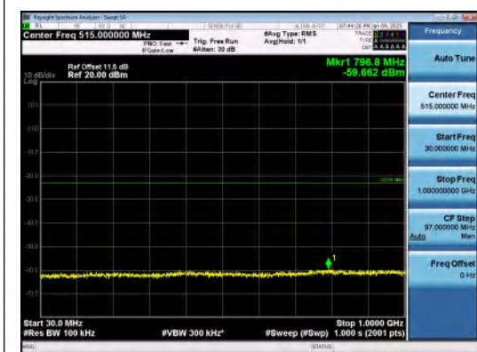
Band66-20MHz-16QAM-132072-1RB#99-30~1000-PASS
