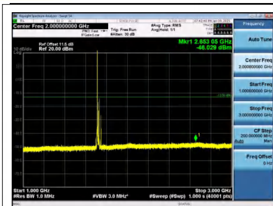
Band66-20MHz-16QAM-132072-1RB#0-1000~3000-PASS
