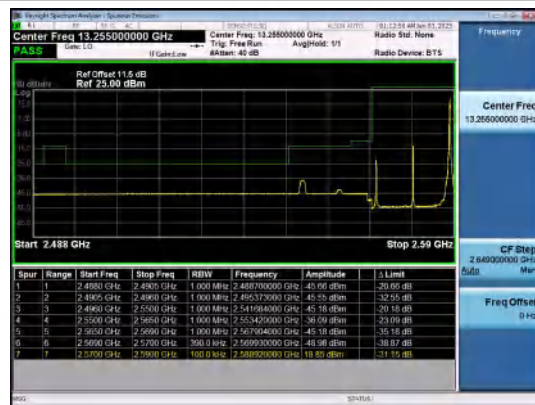
Band38-20MHz-16QAM-37850-1RB#99-PASS
