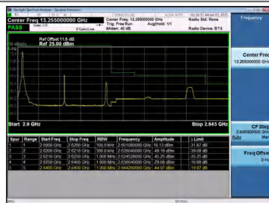
Band38-20MHz-16QAM-38150-1RB#0-PASS
