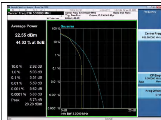
Band26(824-849)-3MHz-16QAM-26915-1RB#0-P
