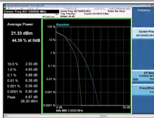
Band26(824-849)-3MHz-16QAM-27025-15RB#0-P
