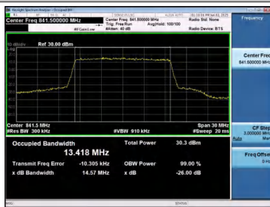
Band26(824-849)-15MHz-16QAM-26965-75RB#0- PASS
