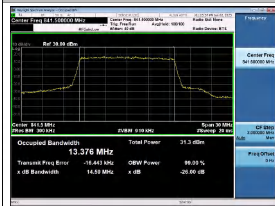
Band26(824-849)-15MHz-QPSK-26965-75RB#0- PASS
