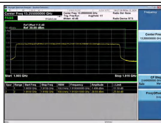
Band25-10MHz-16QAM-26640-50RB#0-PASS
