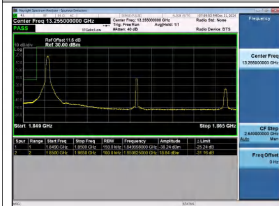
Band25-15MHz-QPSK-26115-1RB#0-PASS
