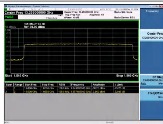
Band25-15MHz-16QAM-26115-75RB#0-PASS
