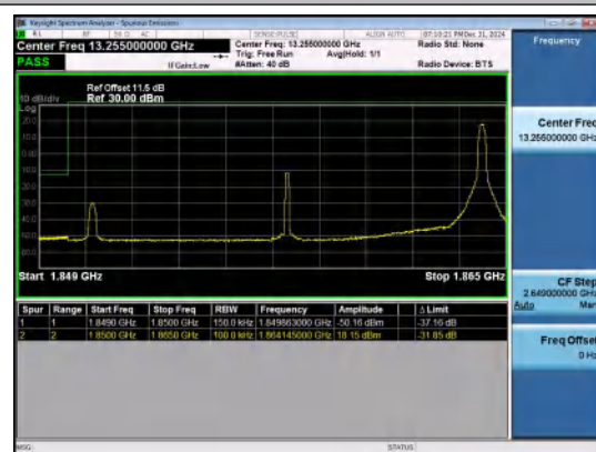
Band25-15MHz-QPSK-26115-1RB#74-PASS
