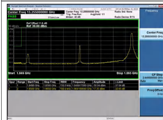
Band25-15MHz-16QAM-26115-1RB#74-PASS
