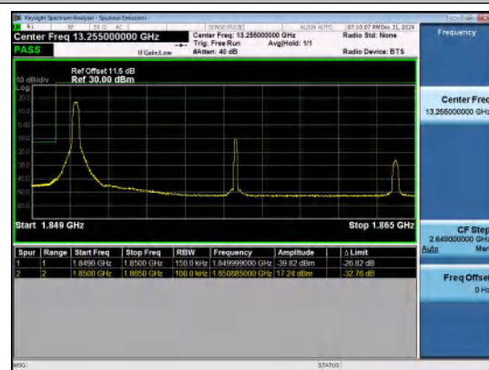
Band25-15MHz-16QAM-26115-1RB#0-PASS
