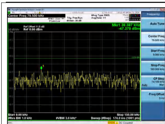
Band12-5MHz-16QAM-23035-1RB#24-0.009~0.15-PASS
