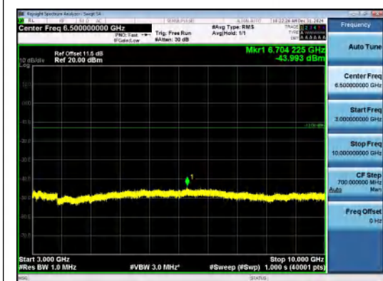
Band12-5MHz-16QAM-23035-1RB#24-3000~10000-PASS
