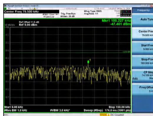
Band12-5MHz-16QAM-23035-25RB#0-0.009~0.15-PASS
