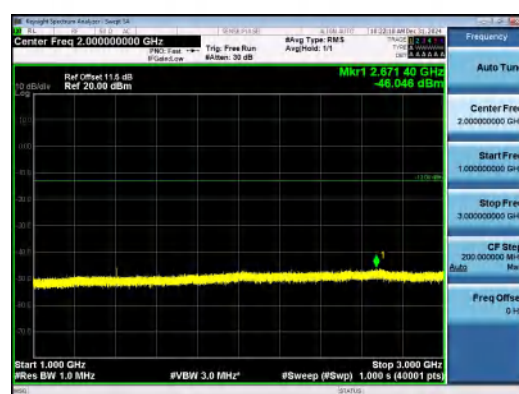
Band12-5MHz-16QAM-23035-1RB#24-1000~3000-PASS
