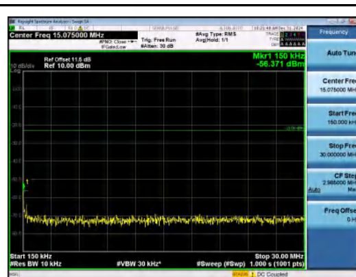
Band12-5MHz-16QAM-23035-1RB#24-0.15~30-PASS
