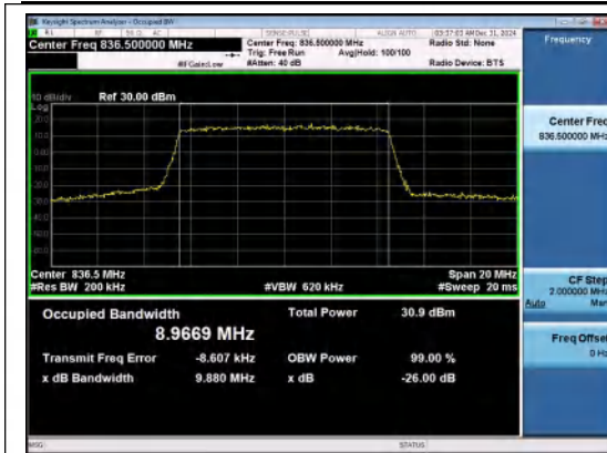
Band5-10MHz-QPSK-20525-50RB#0-PASS
