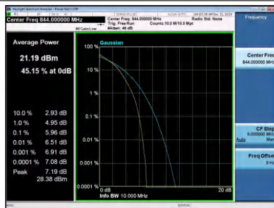
Band5-10MHz-16QAM-20600-50RB#0-PASS
