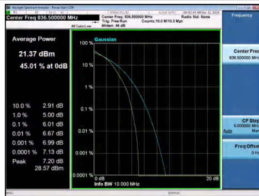
Band5-10MHz-16QAM-20525-50RB#0-PASS
