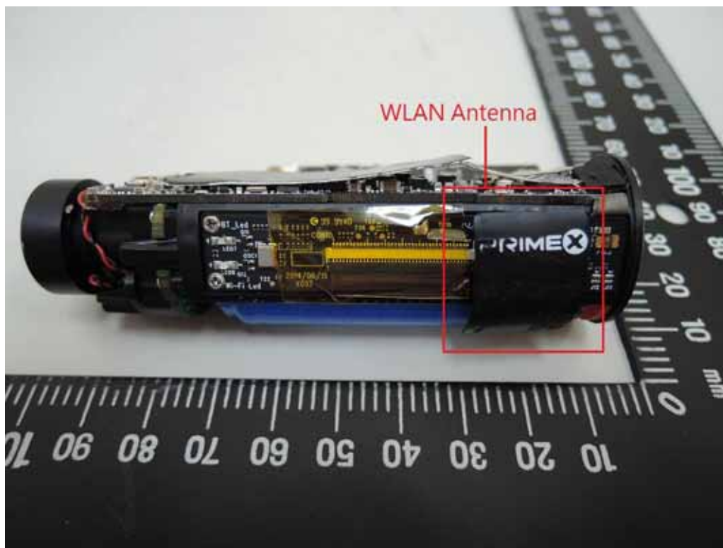
WLAN Antenna - 2
