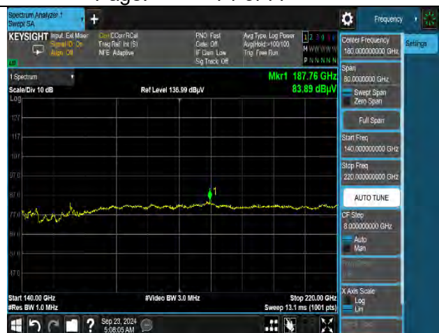
Channel 2 140-220GHz-Vertical
