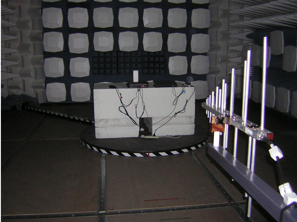
Radiated Emissions (30MHz to 1000MHz)
