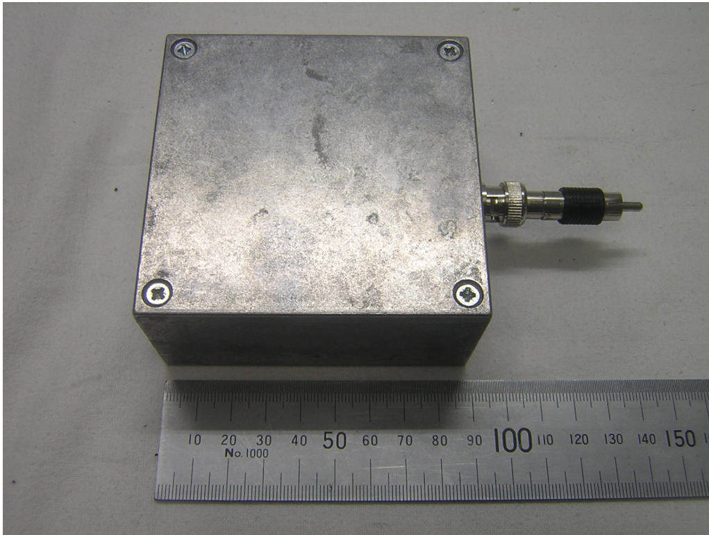
50Ω Termination Box
