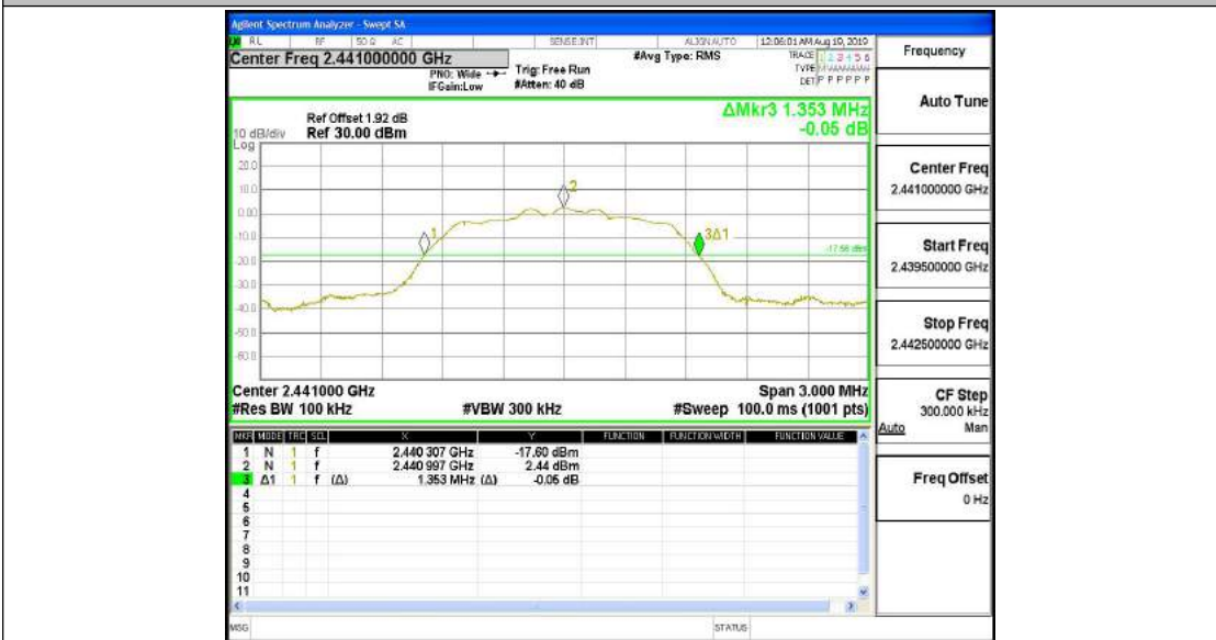
2DH1_Ant1_2441
