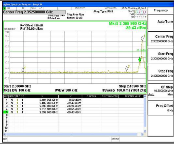
2DH1_Ant1_Low_2402
