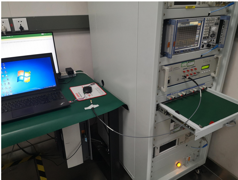
Conducted Test-WIFI
