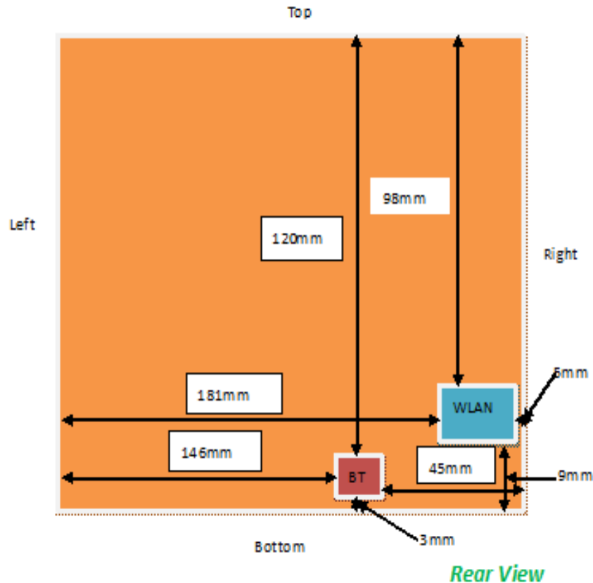
Figure 2: The antenna positions of the DUT
