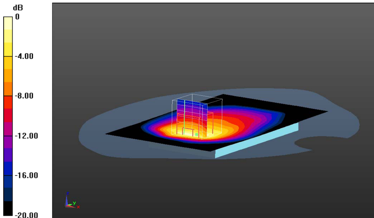
Plot 1: Rear Side (WLAN2450-Middle Channel-Channel 6-2437MHz(1Mbps))
