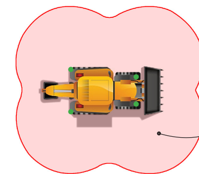
Four Antenna System Fitted to Shovel Loader
