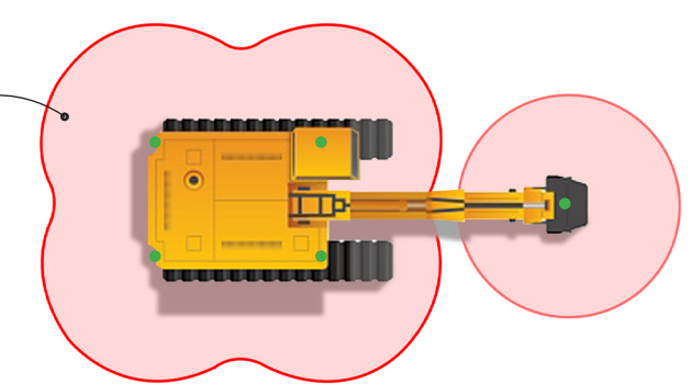
Five Antenna System Fitted to Excavator with Antenna Fitted to Digger Arm
