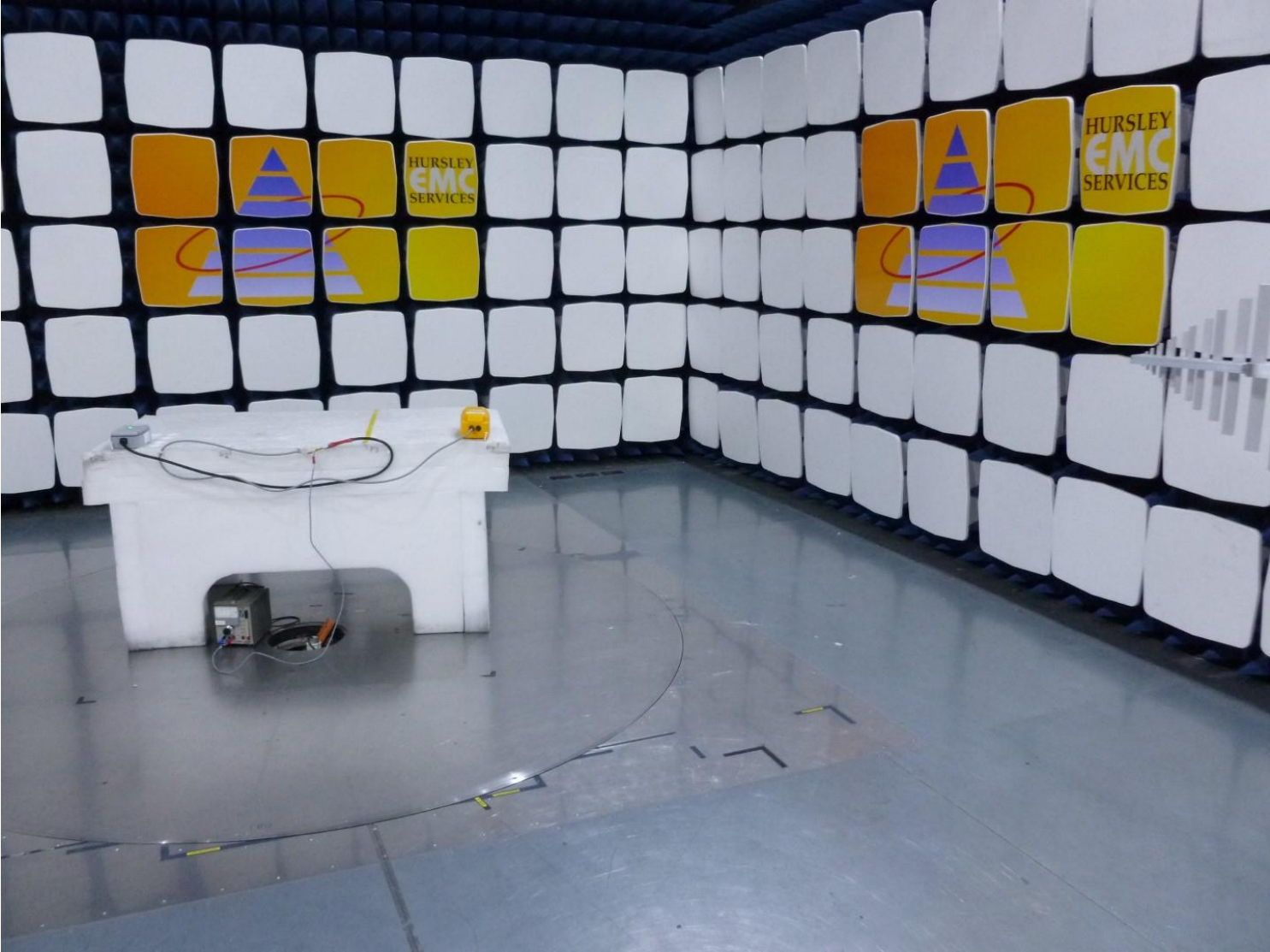
2ACWNZSA6782 Antenna Unit Test Setup Photos
