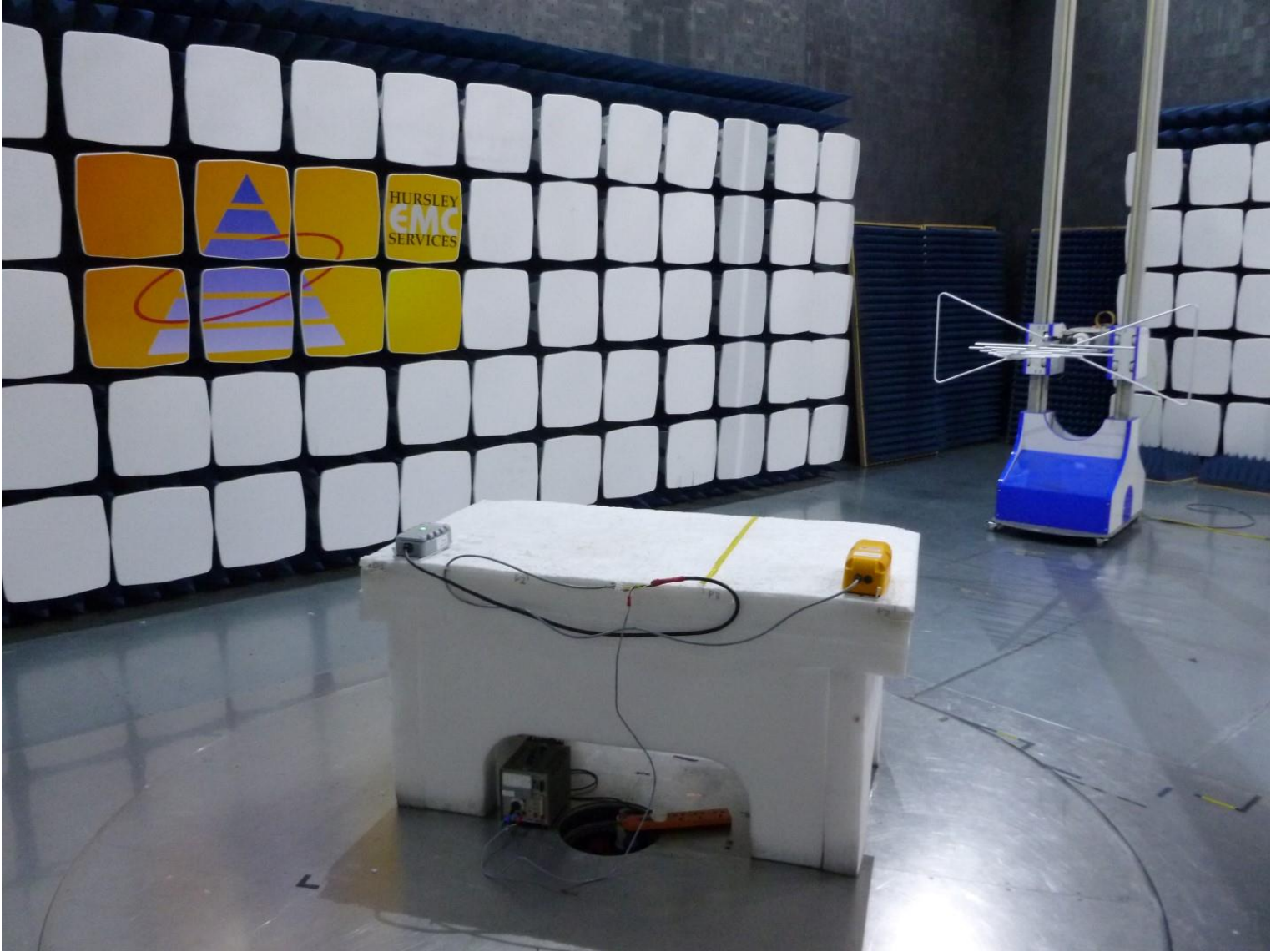
2ACWNZSA6782 Antenna Unit Test Setup Photos
