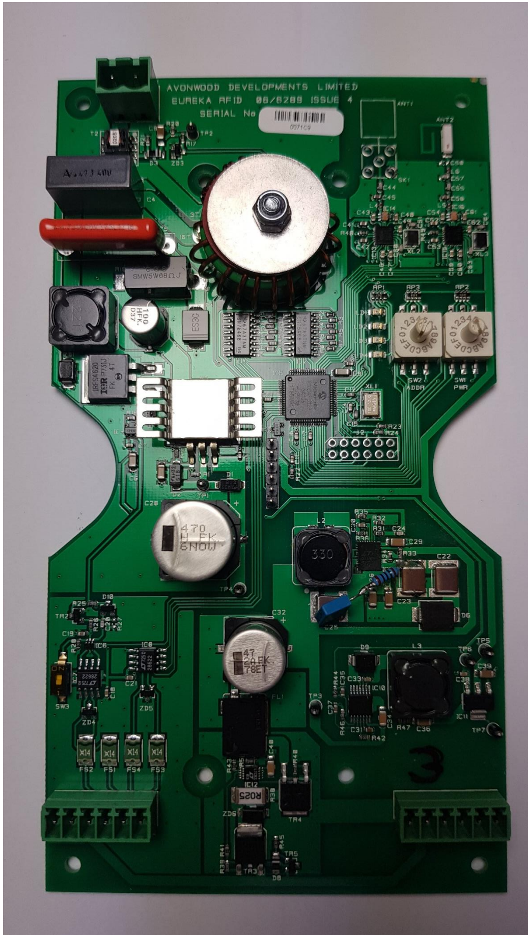
2ACWNZSA6782 - ZoneSafe Antenna Unit Internal Photos
