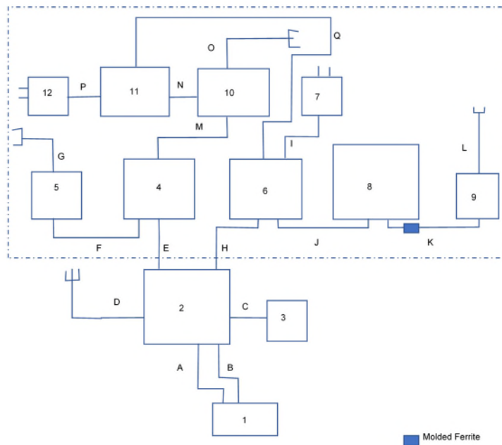
Figure 6-2: EUT Test Setup Diagram – Power Line Conducted Emissions
