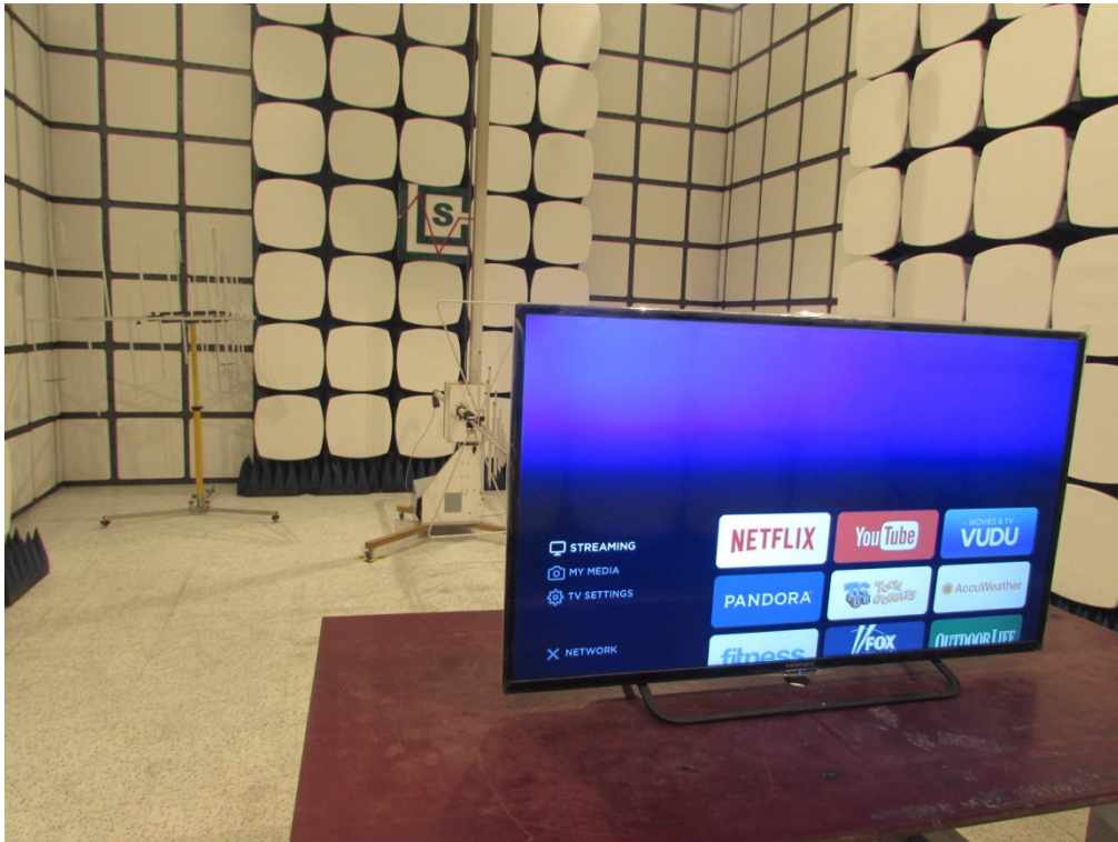
Radiation Test(30-1000MHz)
