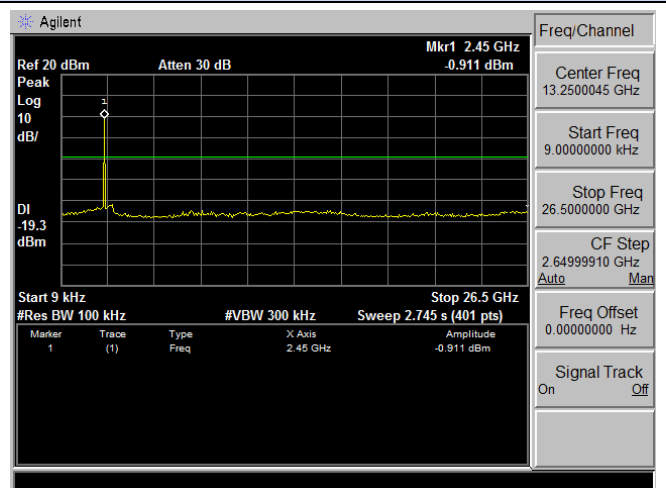
9 KHz – 26.5 GHz
