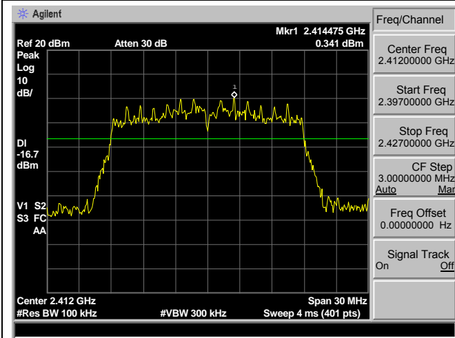
2397 MHz – 2427 MHz
