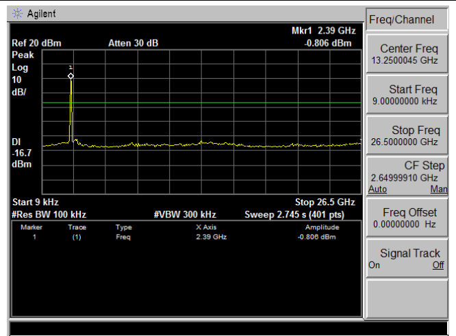
9 KHz – 26.5 GHz
