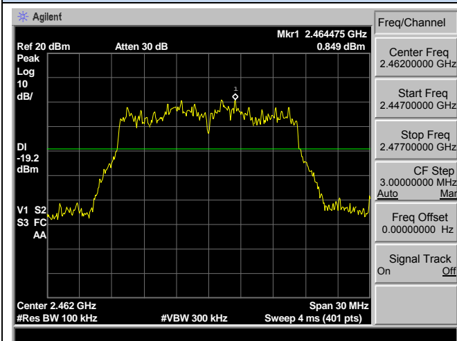
2447 MHz – 2477 MHz
