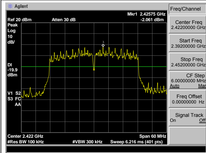
2392 MHz – 2452 MHz
