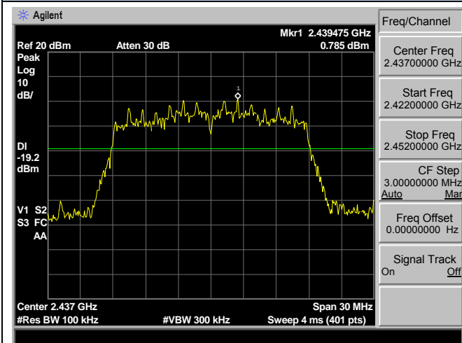
2422 MHz – 2452 MHz
