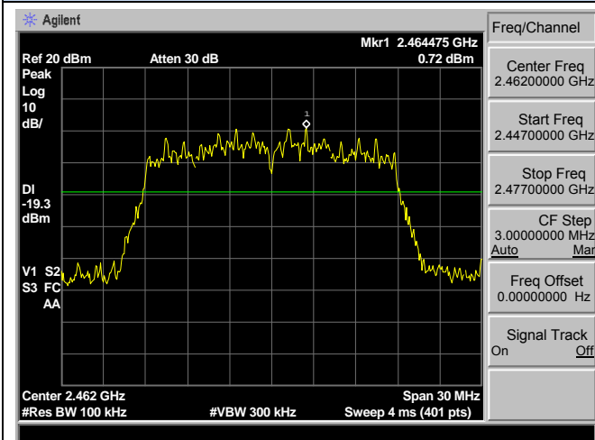
2447 MHz – 2477 MHz
