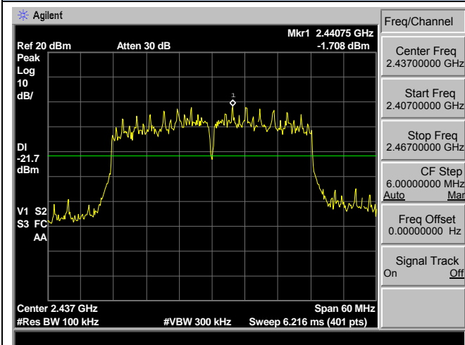
2407 MHz – 2467 MHz
