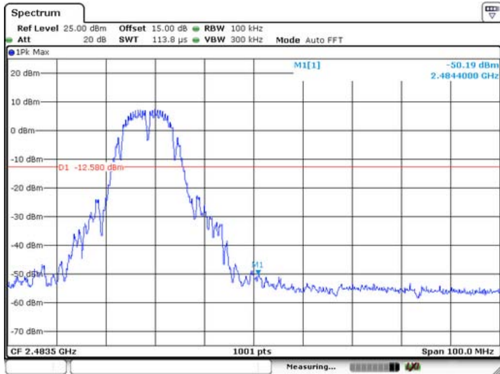
Test Mode: IEEE 802.11g SISO Ant1
