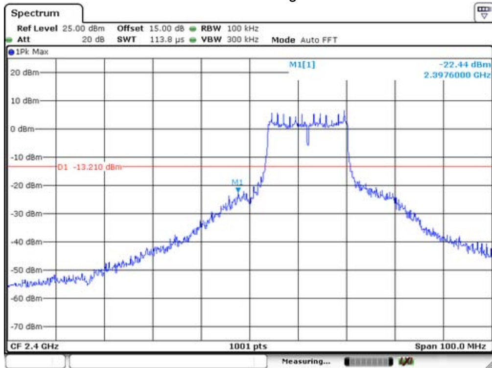
Test Mode: IEEE 802.11g SISO Ant2
