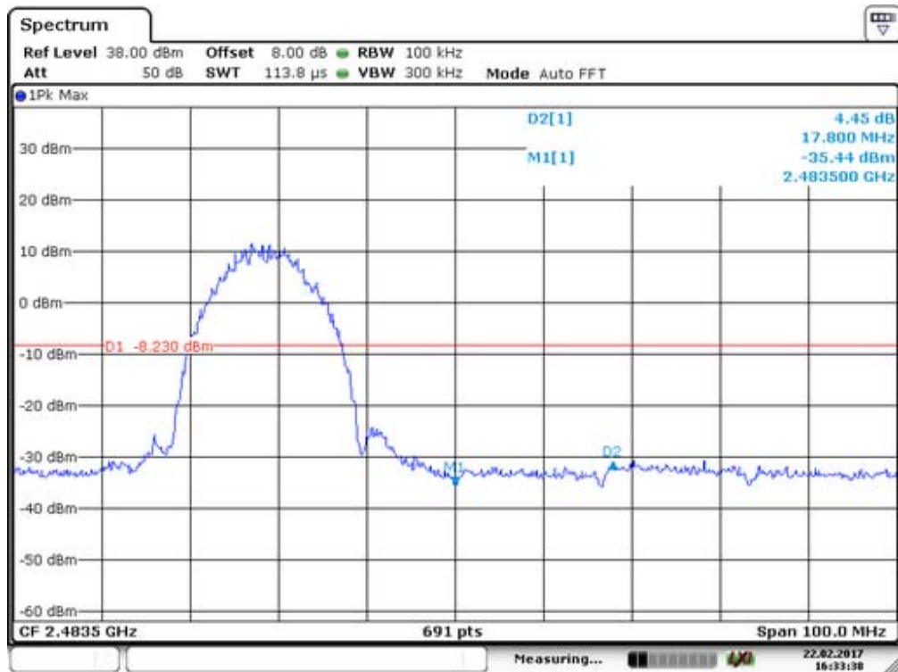
Test Mode: IEEE 802.11b SISO Ant2
