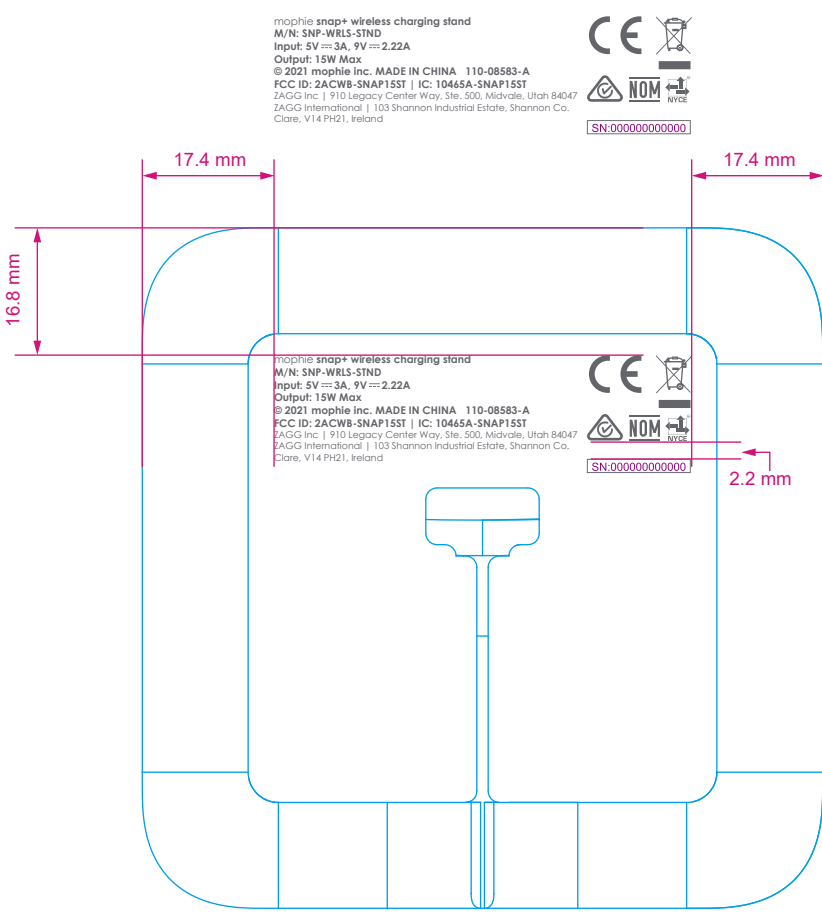
Bottom view
