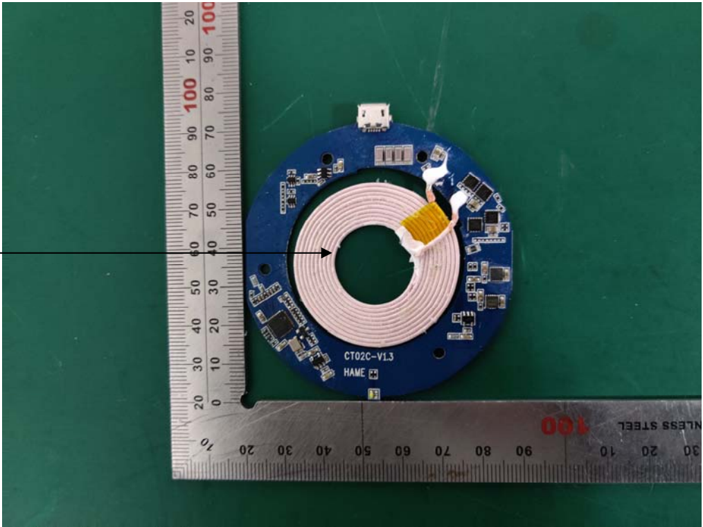
Coil Antenna
