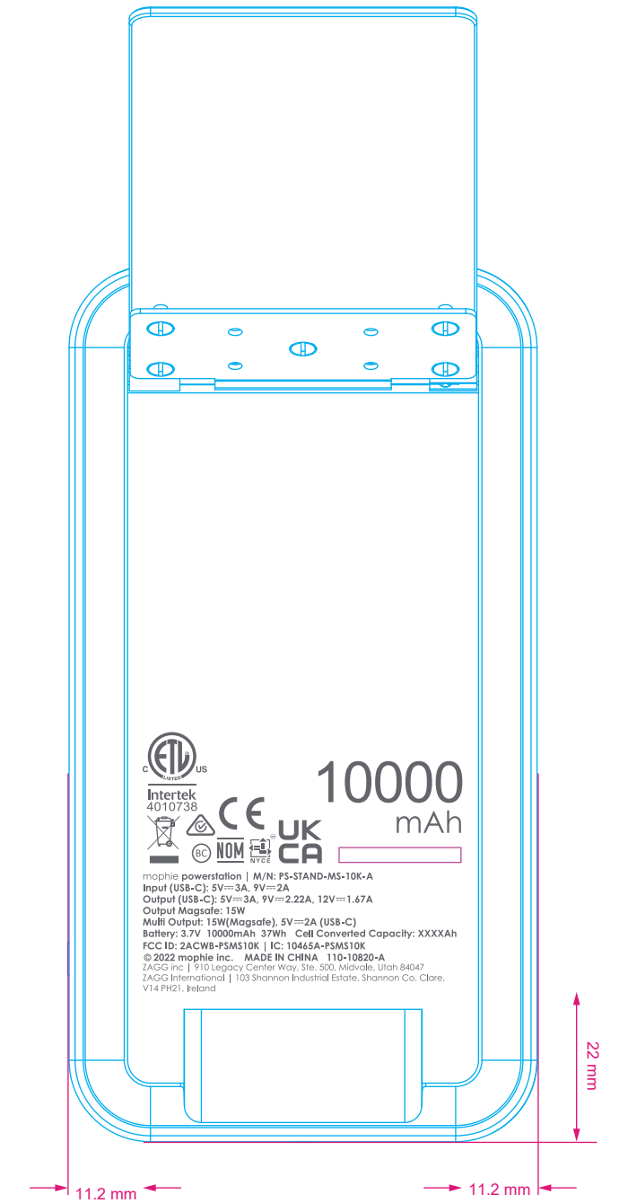
Kickstand rotated 120° back view
