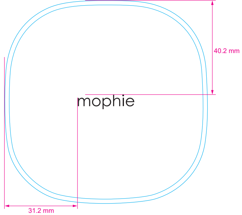
TOP VIEW
