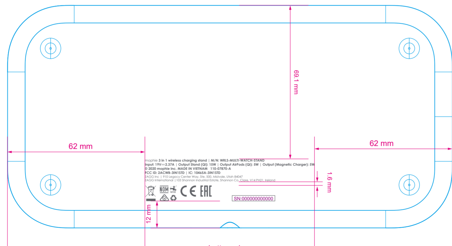
bottom view
