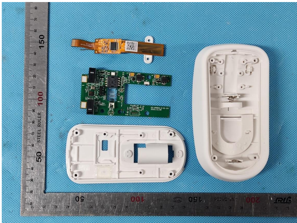
OPEN VIEW OF EUT (Touch-Scroll)
