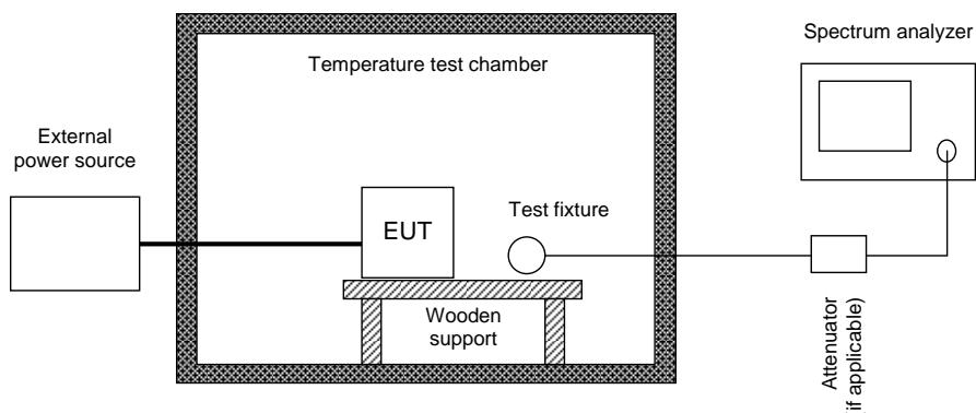
Picture 6: Test setup for carrier frequency stability measurement
