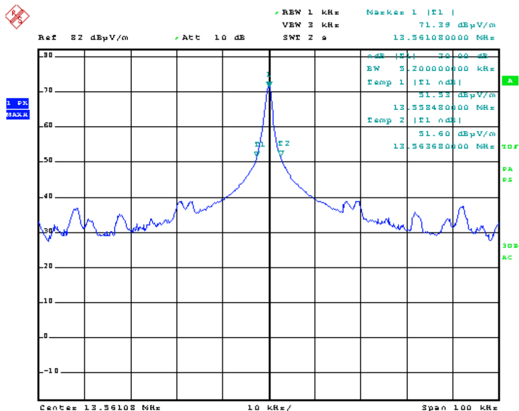
Picture 9: -20 dB emission bandwidth
