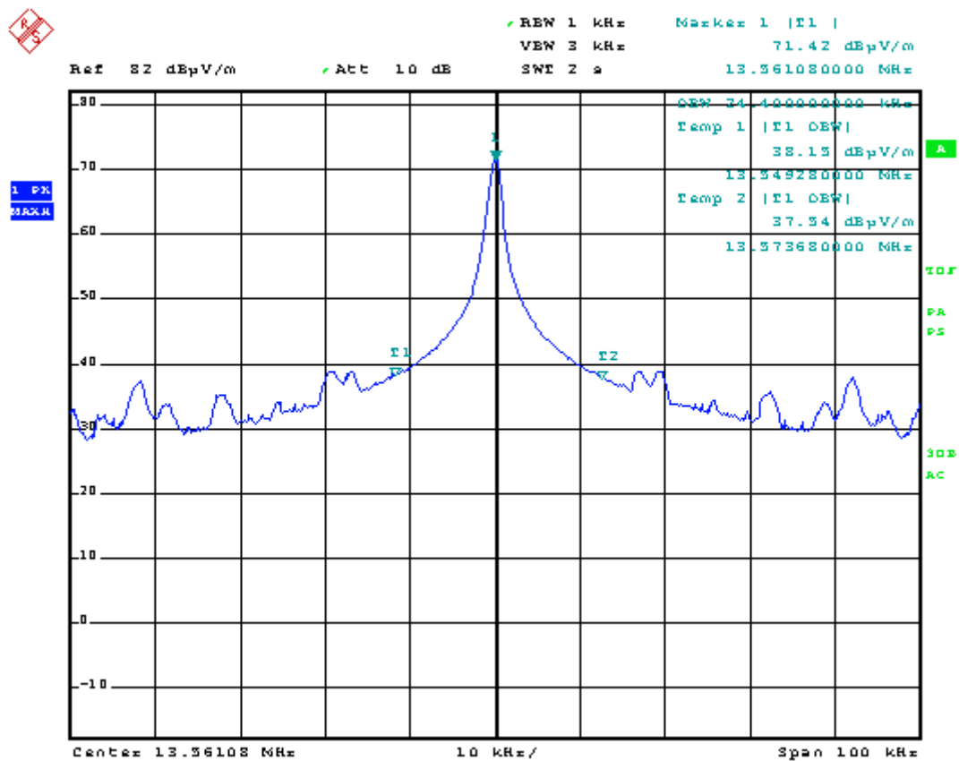
Picture 7: Occupied bandwidth (99 %)
