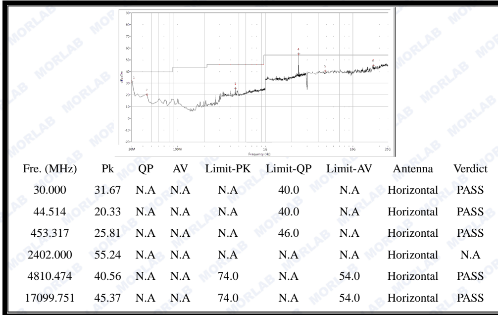
(Antenna Horizontal, 30MHz to 25GHz)
