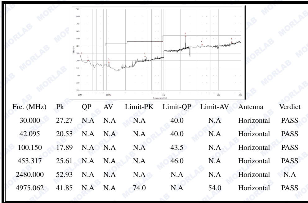
(Antenna Horizontal, 30MHz to 25GHz)
