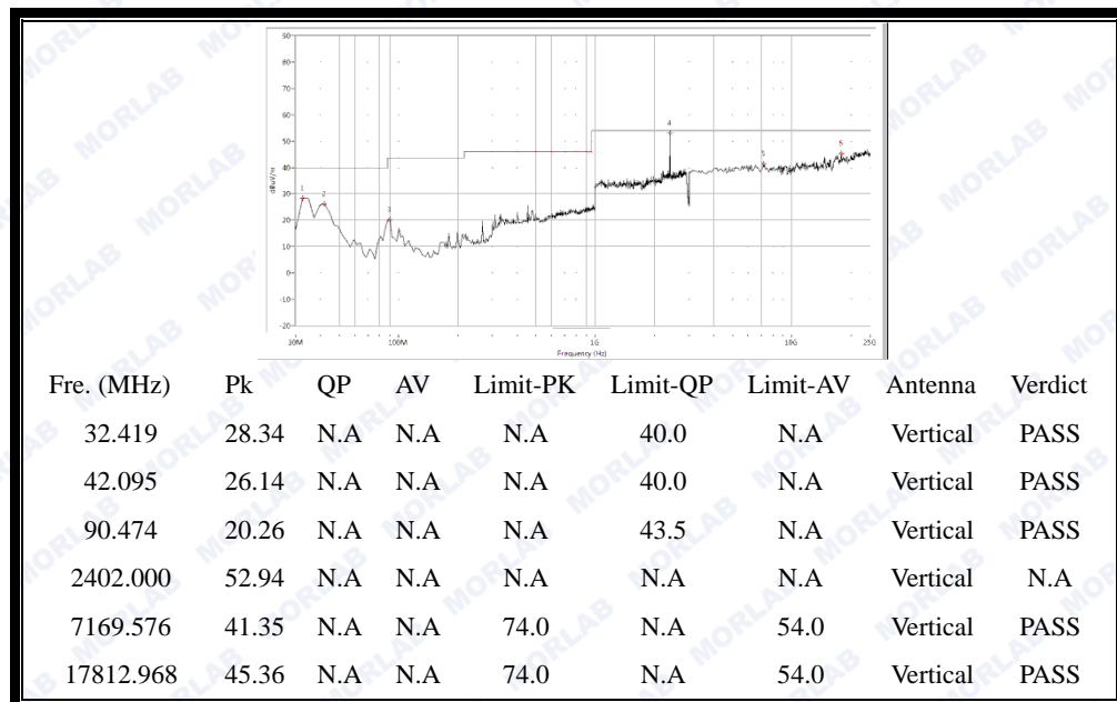
(Antenna Vertical, 30MHz to 25GHz)
