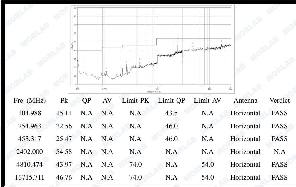
(Antenna Horizontal, 30MHz to 25GHz)
