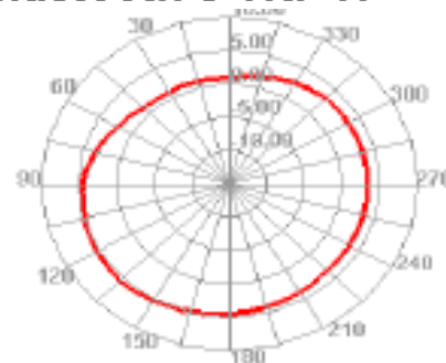
Radiation Pattern Bluetooth 0 TRP H
