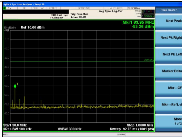
\pi/4 -DQPSK on channel 79
