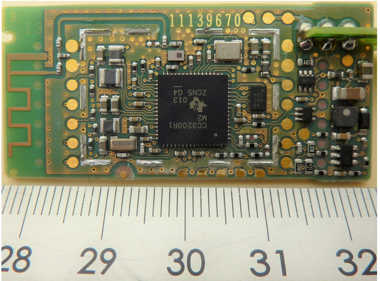
EUT Shielding removed
