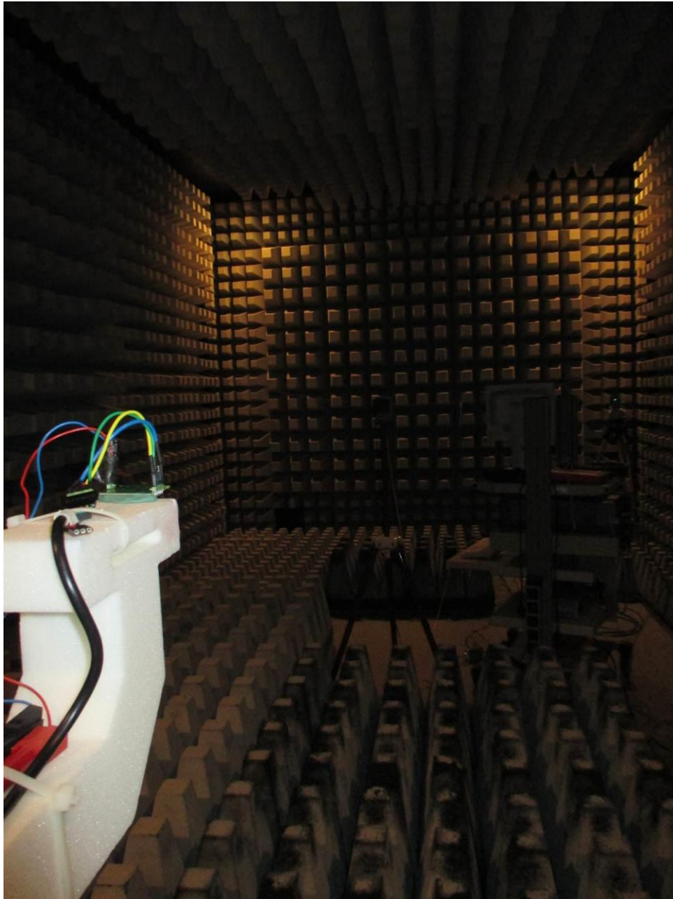
150729_15: Test setup - Radiated emission (fully anechoic chamber)
