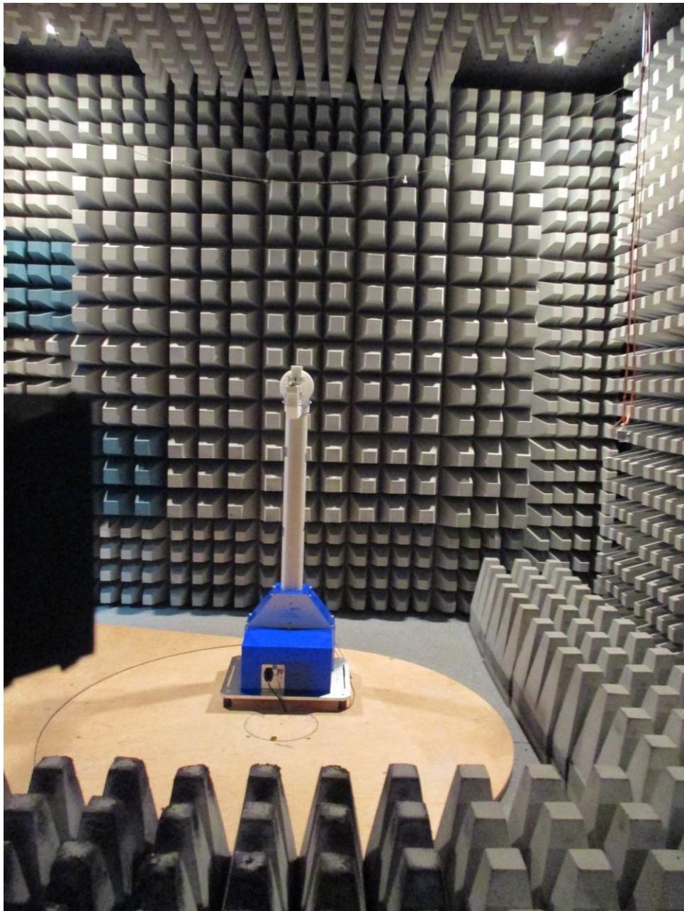
150729_14: Test setup - Radiated emission (fully anechoic chamber)
