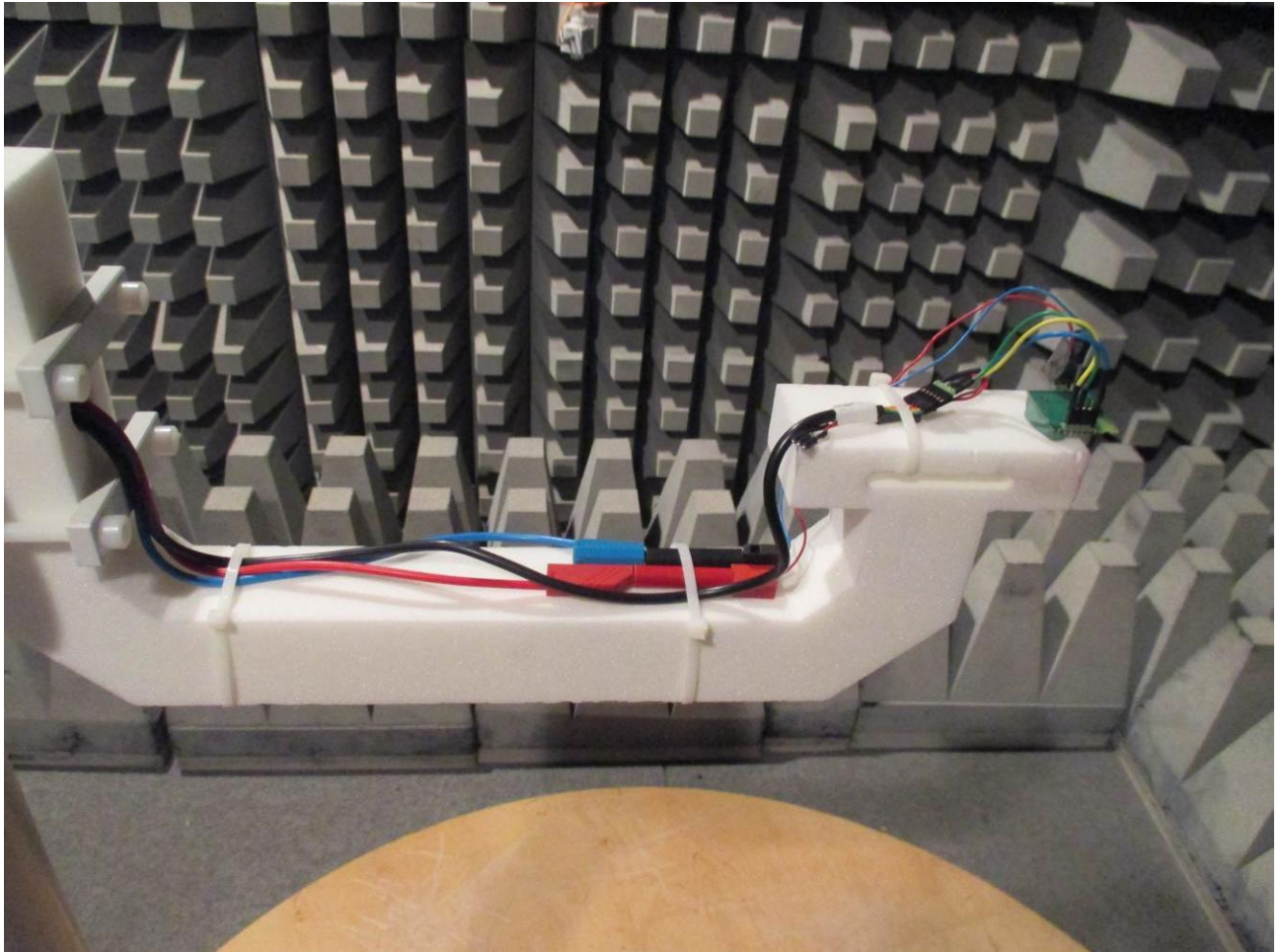
150729_13: Test setup - Radiated emission (fully anechoic chamber)
