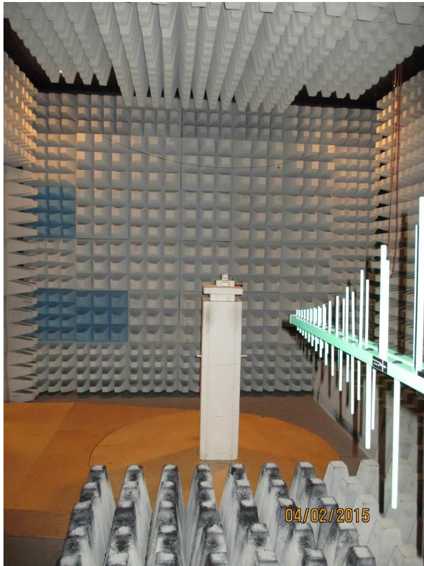
150729_08: Test setup - Radiated emission < 1 GHz (fully anechoic chamber)
