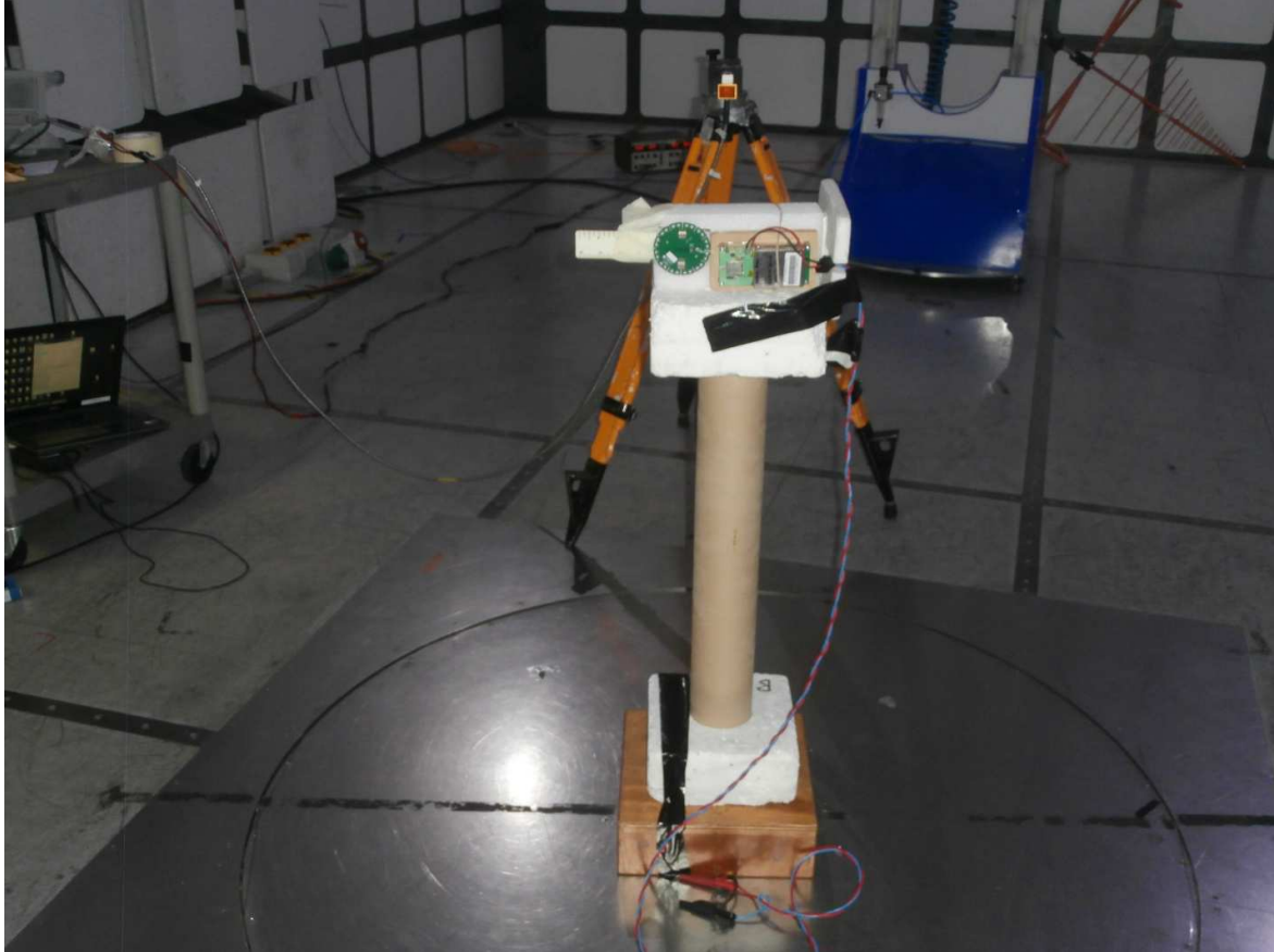
Radiated Emissions 18 GHz to 25 GHz
