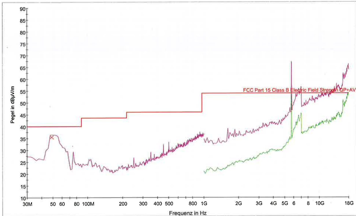
— PK+_MAXH@Naim Feld\NP800_WLAN5G_149153_F1 — AVG_MAXH@Naim Feld — FCC Part 15 Class B Electric Field Strength QP+AV x PK+_MAXH@Naim Feld QuasiPeak@Naim Feld
