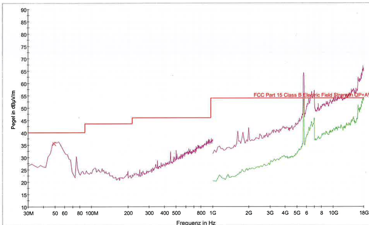
— PK+_MAXH@Naim Feld\NP800_WLAN5G_132144_F1 — AVG_MAXH@Naim Feld — FCC Part 15 Class B Electric Field Strength QP+AV x PK+_MAXH@Naim Feld QuasiPeak@Naim Feld
