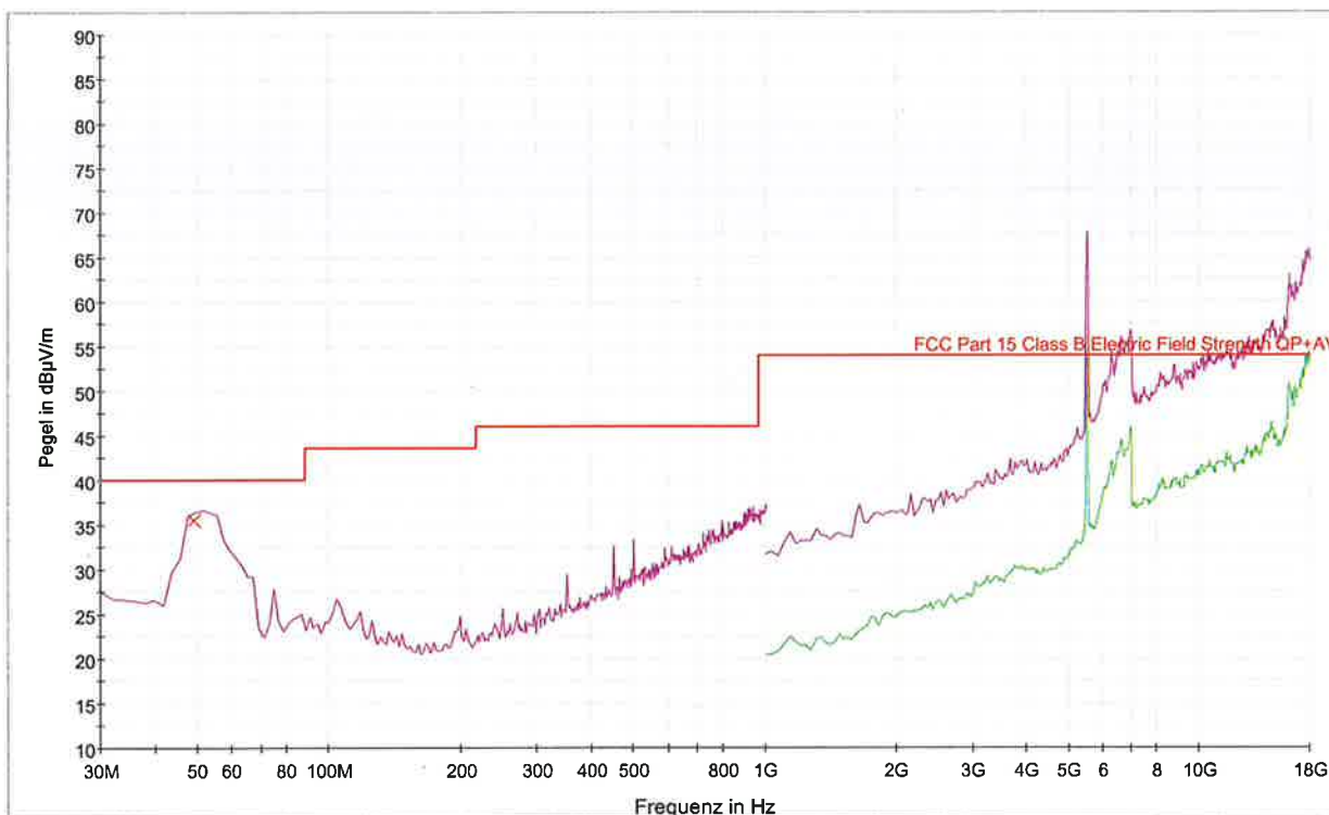
— PK+_MAXH@Naim Feld\NP800_WLAN5G_100104_F1 — AVG_MAXH@Naim Feld — FCC Part 15 Class B Electric Field Strength QP+AV x PK+_MAXH@Naim Feld QuasiPeak@Naim Feld
