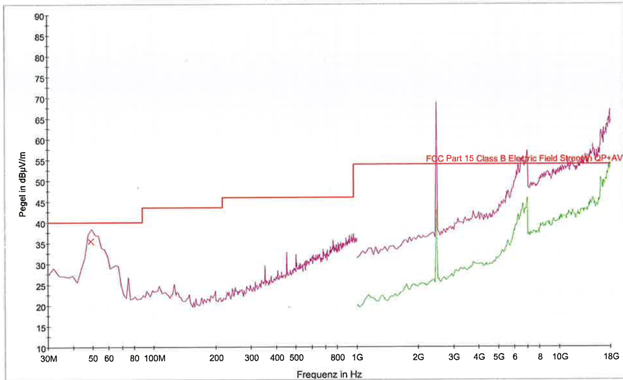
— PK+_MAXH@Naim Feld\NP800_BT_EDR_78_F1 — AVG_MAXH@Naim Feld — FCC Part 15 Class B Electric Field Strength QP+AV x PK+_MAXH@Naim Feld QuasiPeak@Naim Feld
