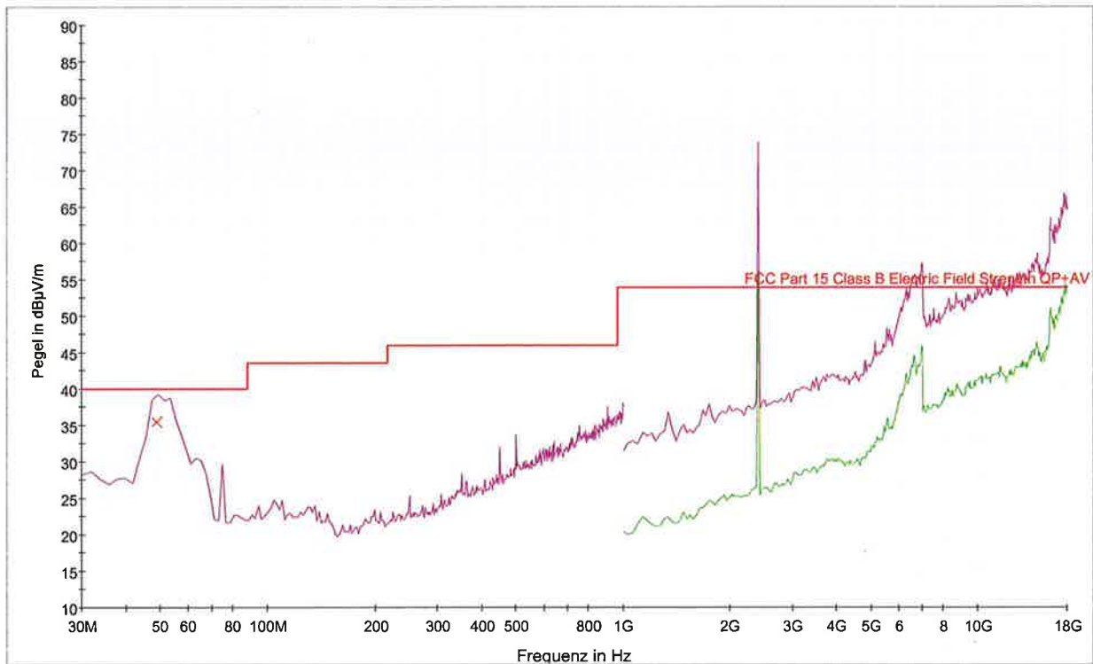
— PK+ _MAXH@Naim Feld\NP800_BT_BDR_0_F1 — AVG_MAXH@Naim Feld — FCC Part 15 Class B Electric Field Strength QP+AV x PK+ _MAXH@Naim Feld QuasiPeak@Naim Feld
