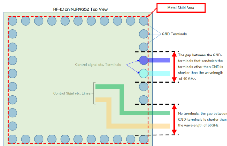
Fig. 2:Top View
