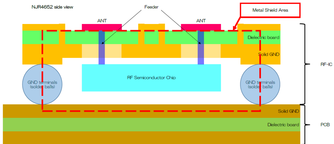
Fig. 1:Side View
