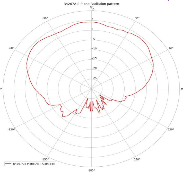
Radiation Pattern
