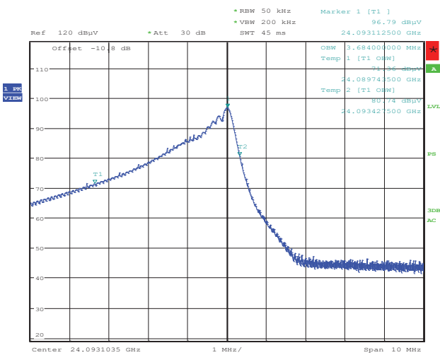
Figure 7: 99% Bandwidth, Configuration 2
