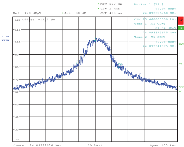
Figure 6: 99% Bandwidth, Configuration 1
