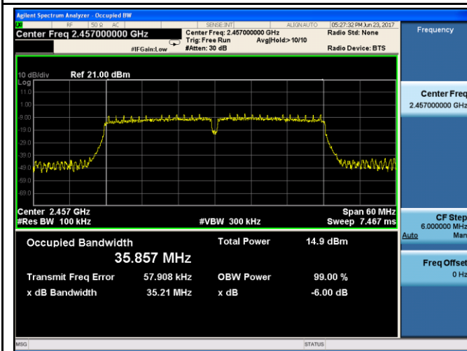
802.11n40 6dB Bandwidth - CH 12
