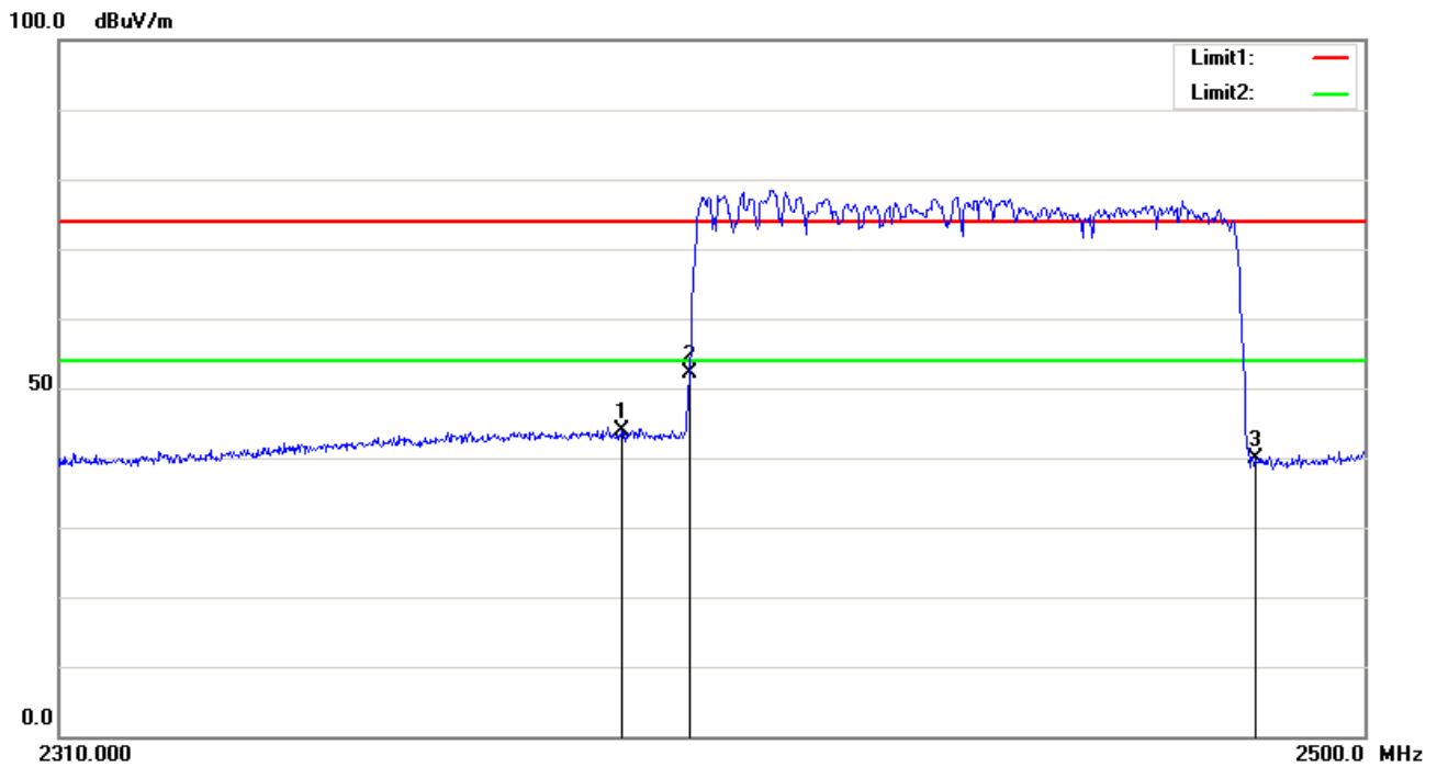
8-DPSK -Hopping-Horizontal
