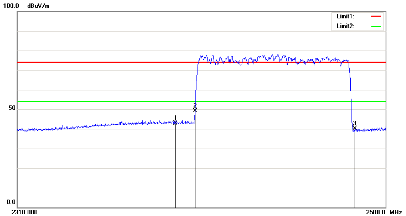
8-DPSK -Hopping-Vertical
