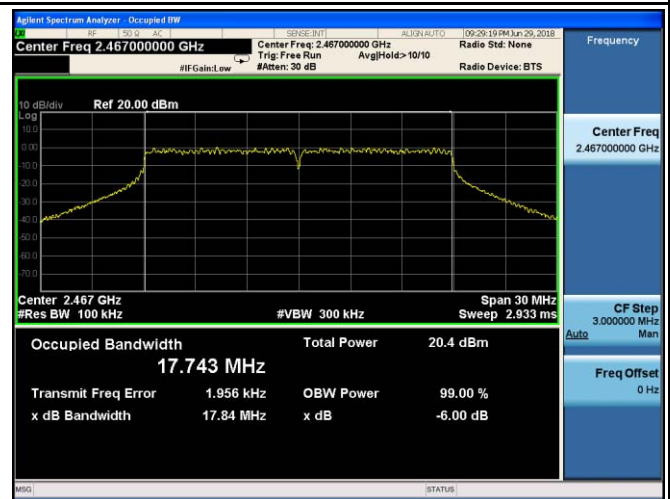
802.11n20 6dB Bandwidth - CH 12
