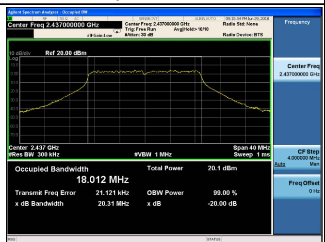
802.11n20 20dB Bandwidth - CH 6
