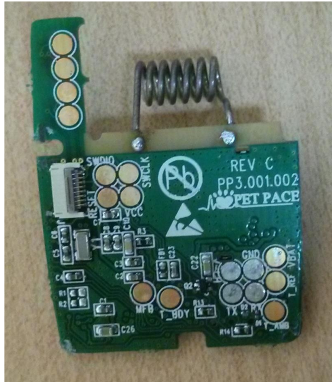
Figure 3 - Collar Main PCB PS
