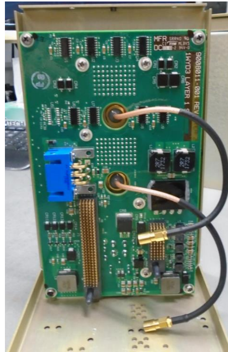
Figure 8: NXT-800 Rear Interconnect Assembly
