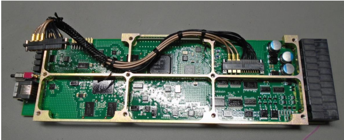
Figure 1: NXT Processor Circuit Card Top View
