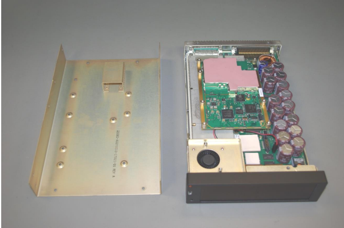
Figure 1: NGT-9000D+ Top View with Top Cover Removed
