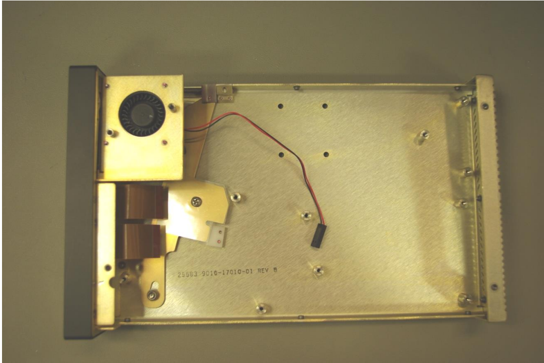
Figure 6: NGT-9000D+ with GPS-UAT CCA and Main CCA Removed
