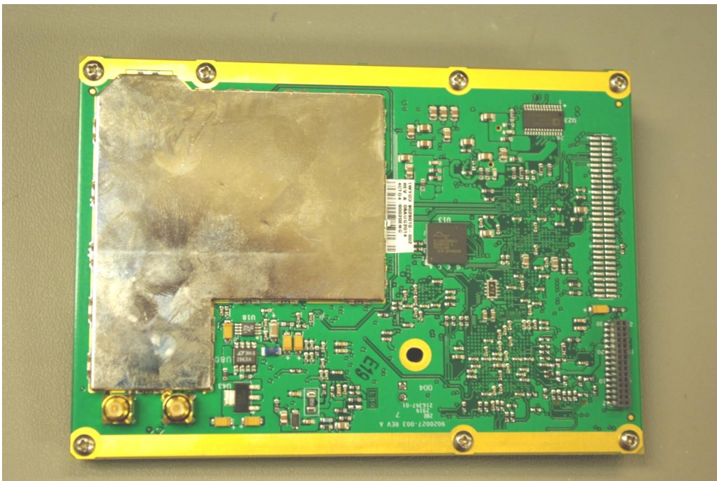
Figure 5: GPS-UAT CCA Bottom Side, common to both the NGT-9000D+ and NGT-9000RD+
