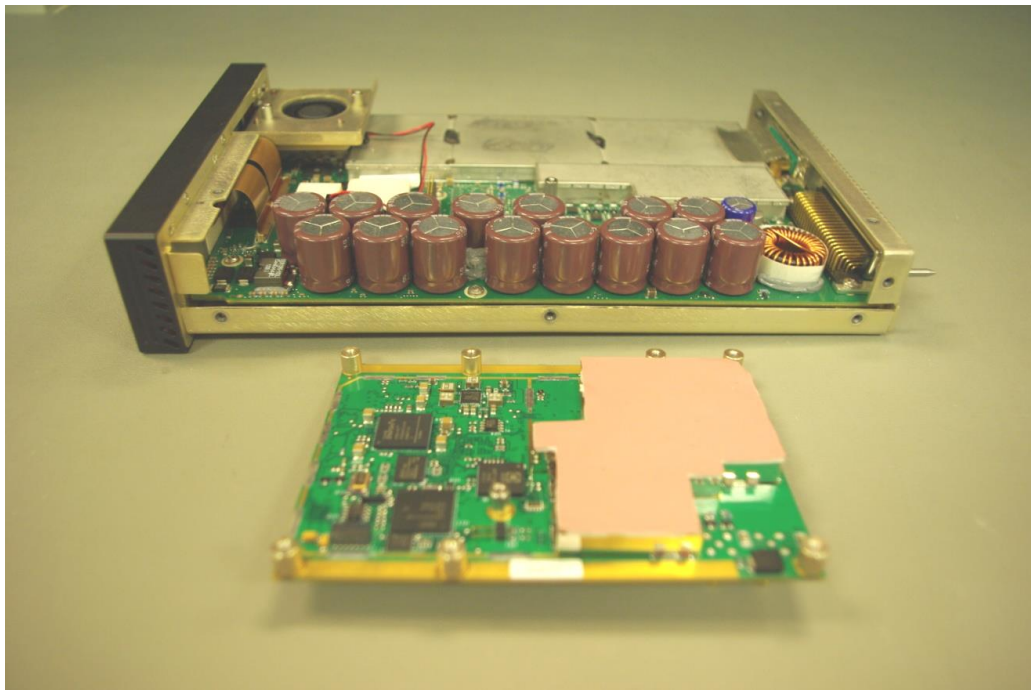
Figure 3: NGT-9000D+ with GPS-UAT CCA Removed
