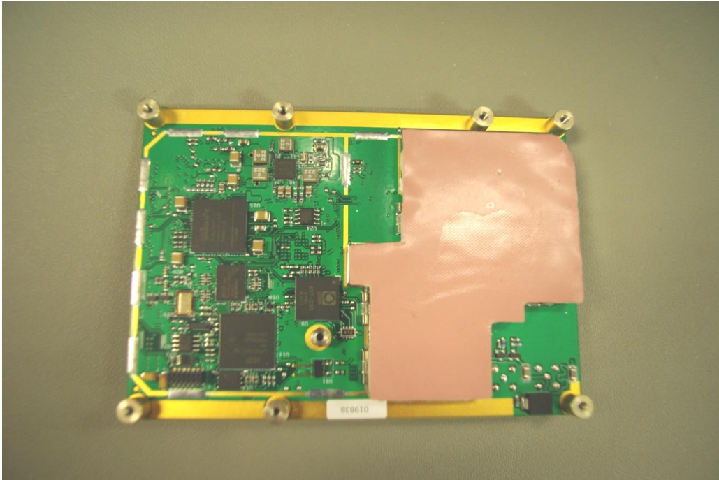
Figure 4: GPS-UAT CCA Top Side, common to both the NGT-9000D+ and NGT-9000RD+
