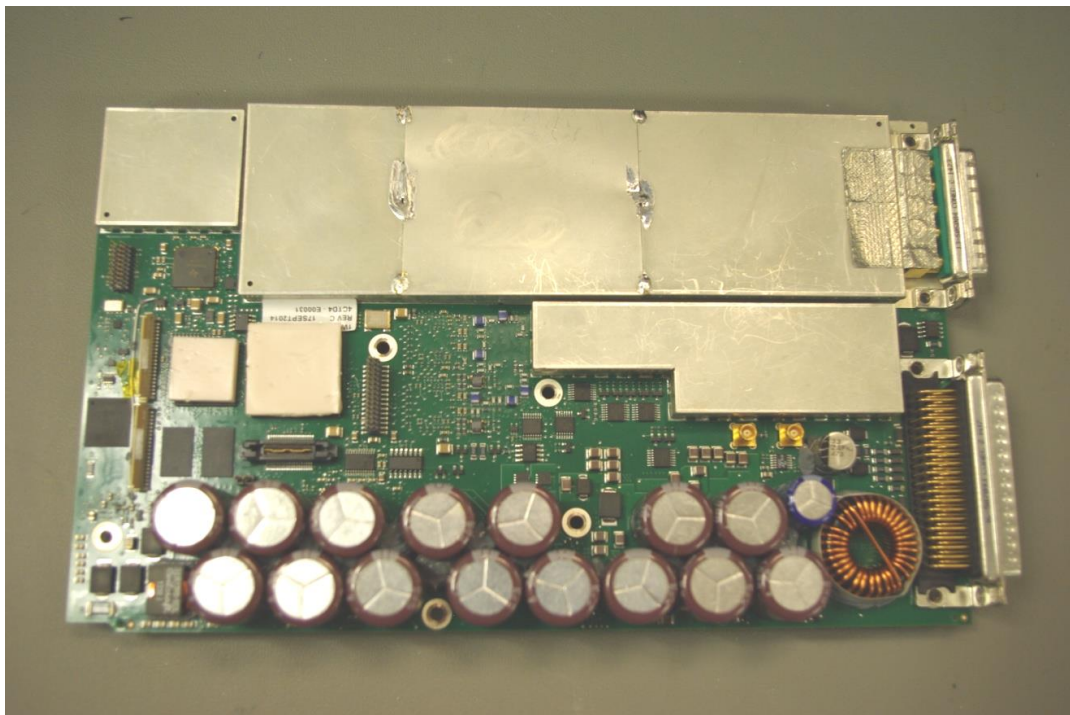
Figure 7: NGT-9000 Main CCA Top Side, common to both the NGT-9000D+ and NGT-9000RD+
