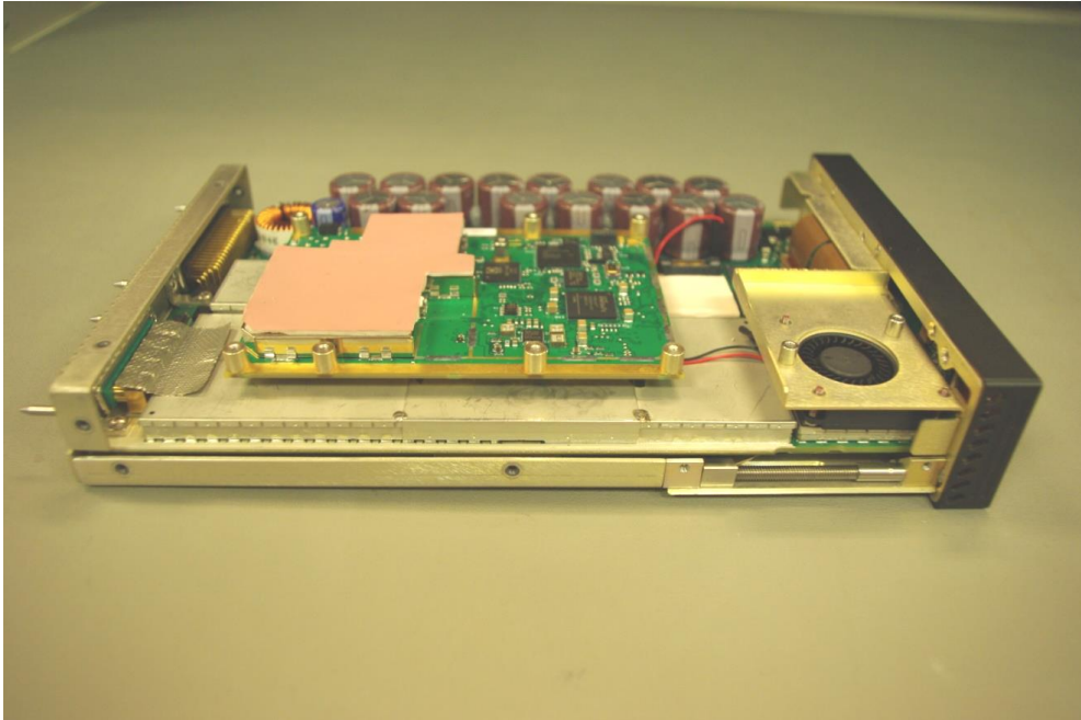
Figure 2: NGT-9000D+ Side View With Top Cover Removed
