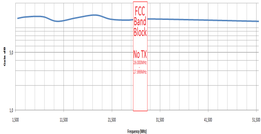
MLA100 Typical Gain vs Frequency
